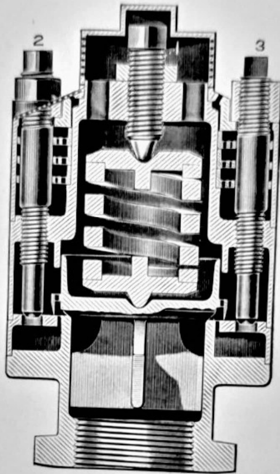
SECTIONAL VIEW.
