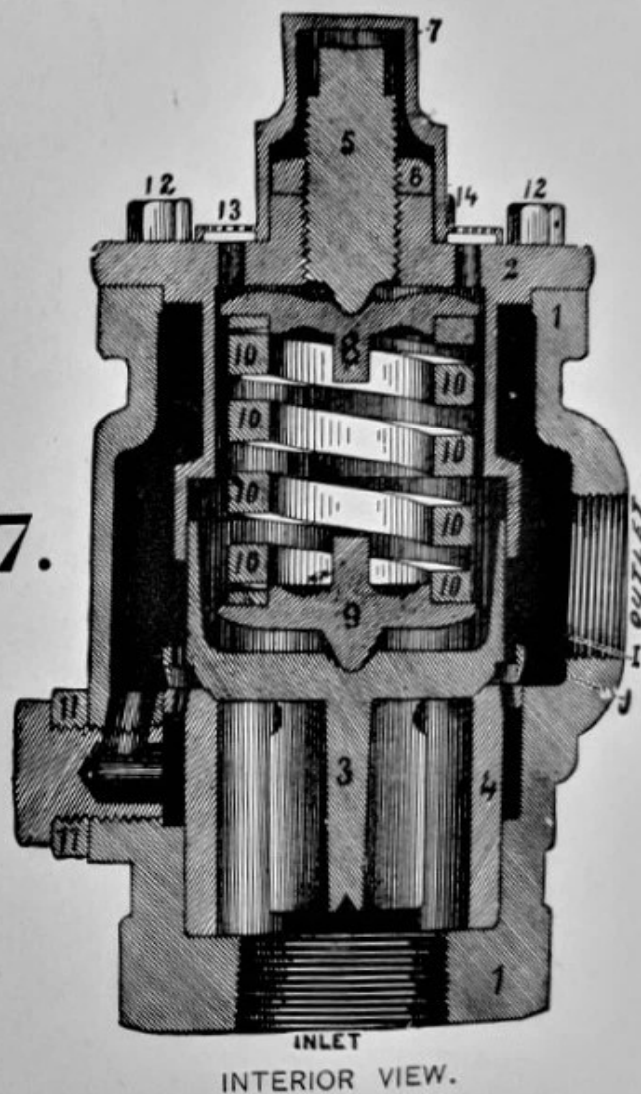
BLOW-BACK VALVE.
