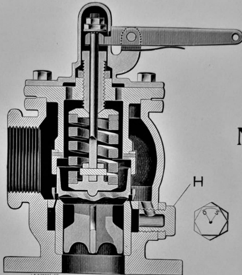
SECTIONAL VIEW.
